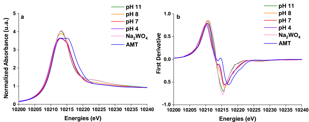
Figure 4. (a) W L_3 -edge XANES normalized spectra, (b) first derivative of (a) of reference tungstate precursors in aqueous solution: ammonium metatungstate AMT and sodium tungstate \text{Na}_2\text{WO}_4 as well as tungstate-mannose aqueous solution at different pH values. [W] = 0.1 \text{ mol.L}^{-1} , [\text{Mannose}] = 0.1 \text{ mol.L}^{-1} . * the experiments were conducted at such low tungsten concentration to prevent fluorescence phenomena. The effect of changing tungsten and mannose concentrations while conserving the same W/sugar ratio was almost ineffectual for the amount of complexed tungsten (See Table S10 in the Supporting Information ).
