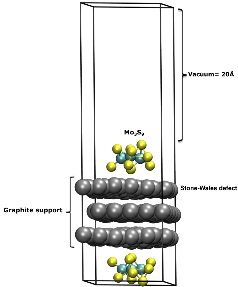
Figure 1: (a) \text{Mo}_3\text{S}_9 nanocluster with the labels of the atoms, (b) the top-most layer of graphite support with a Stone-Wales defect and \text{Mo}_3\text{S}_9 adsorbed and (c) symmetric \text{Mo}_3\text{S}_9 supported on graphite. The adsorption configuration shown is the most stable one. The color code for atoms is white for H; red for O; silver for C; yellow for S and greenish for Mo.
