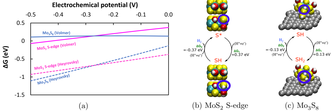
Figure 5: (a) Variation of \Delta G_1 , the Volmer step and \Delta G_2 , the Heyrovsky step as a function of the electrochemical potential for \text{MoS}_2 S-edge and \text{Mo}_3\text{S}_8 , (b) the cycle between \text{SH} and \text{S} to release \text{H}_2 on \text{MoS}_2 S-edge at 0 V and (c) the cycle between \text{SH}_2 and \text{SH} to release \text{H}_2 on \text{Mo}_3\text{S}_8 at 0 V. The color code for atoms is white for H; red for O; silver for C; yellow for S and greenish for Mo. See Fig. S13 for the quantification of the number of electrons that are transferred together with the protons.
