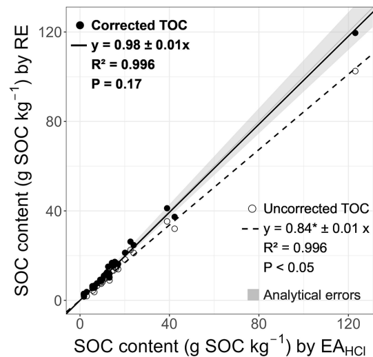
Figure 4. Plot of the SOC content estimated by the uncorrected and corrected TOC parameters of the RE analysis on one aliquot vs. the SOC content estimated by EA_{HCl} on one aliquot for the 30 soils of the first panel. The corrected TOC vs. EA_{HCl} (bold line) and uncorrected TOC vs. EA_{HCl} (dashed line) linear regressions are provided with their coefficient of determination ( R^2 ). For both regressions, the slopes were significantly different from 0 ( p value ( P ) < 0.001 ) but not the intercepts ( P > 0.01 ). The p values presented on the graph indicate the significance of the difference between the slope and 1. * The slope of the regression was significantly different from 1 ( P < 0.05 ). The grey area, centred around the grey line y = x , represents the analytical error in the two methods.
