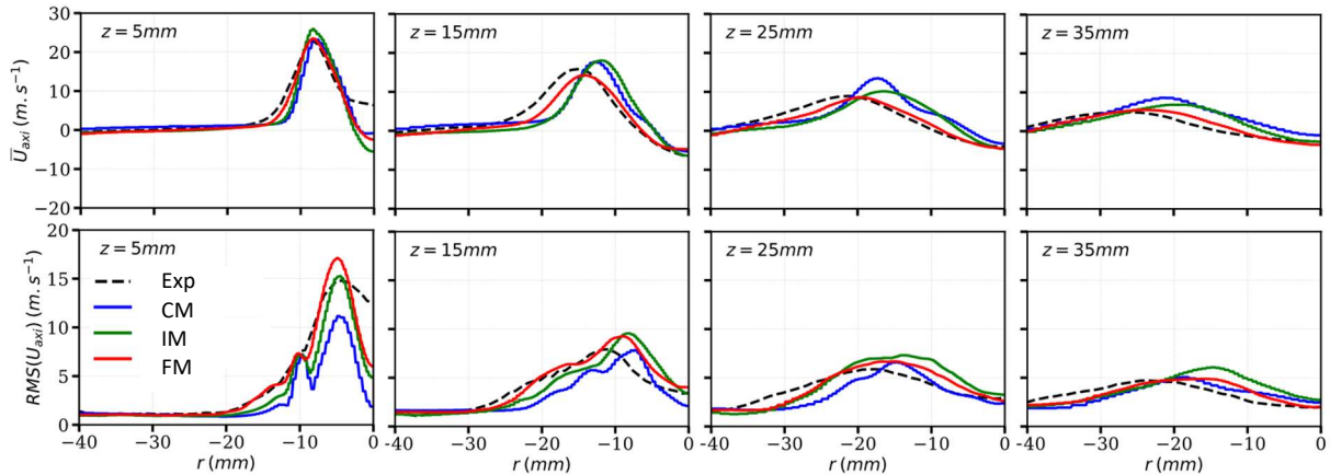
Figure 6. Radial profiles of the axial velocity and the corresponding RMS.
