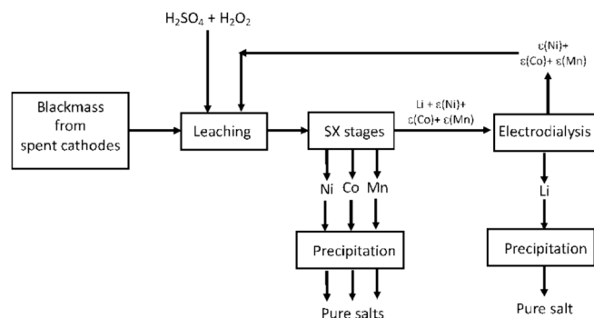
Fig. 23. Principles behind the use of ED in hydrometallurgical systems for generating high-grade lithium salts. Reprinted with permission from [466] (CC-BY MDPI).
