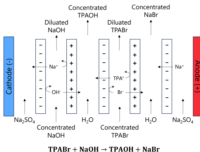
Fig. 18. Schematic principles of the ED metathesis process to prepare tetrapropyl ammonium hydroxide (TPAOH).
