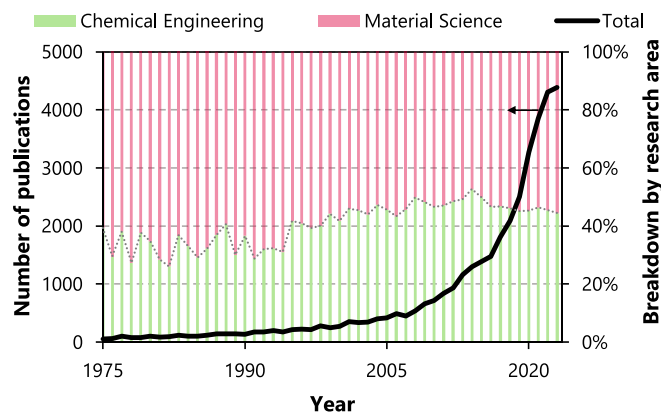
Fig. 1. Number of research articles when searching for the term 'Electrodialysis' as well as the distribution of search fields by query at Digital Science. (1975–2023) Dimensions available from https://app.dimensions.ai . Accessed on 2024/01/10, under license agreement.
