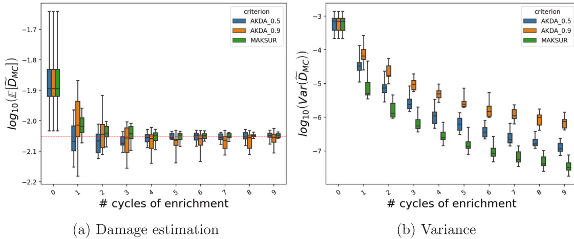
Fig. 16. Evolution of the damage estimation and of the variance of the estimator during the 9 first cycles of enrichment with n_{enr} = 10 .
