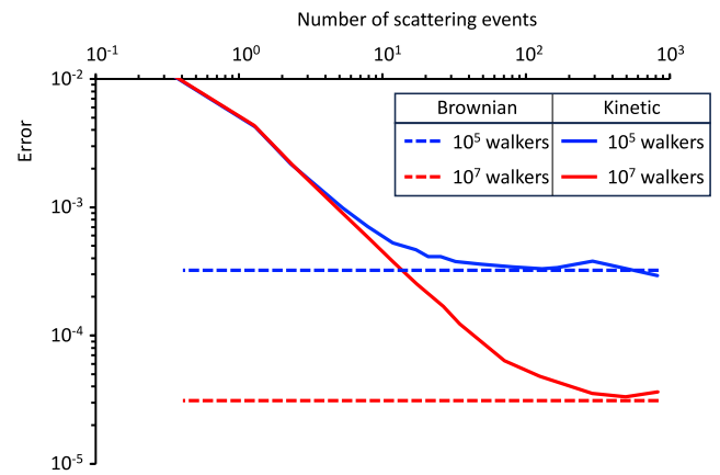
Fig. 3. Behavior of the errors with respect to N_{MC} and f for the Poissonian path and to N_{MC} and \Delta t_{ref} for the Brownian one quantified in terms of total scattering events.
