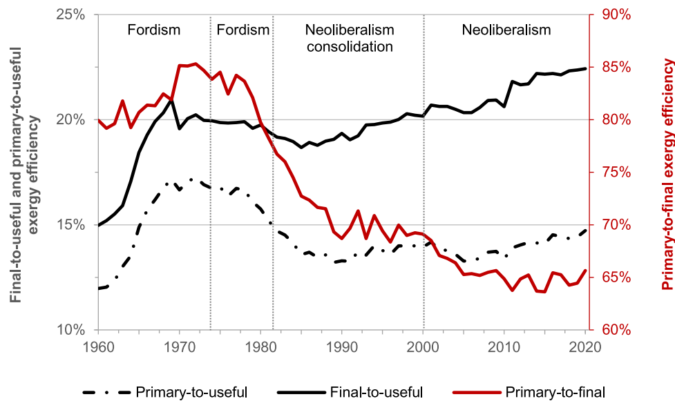
Fig. 5. Thermodynamic efficiency in France (1960–2020). Source: authors, based on data from Brockway et al. (2024).
