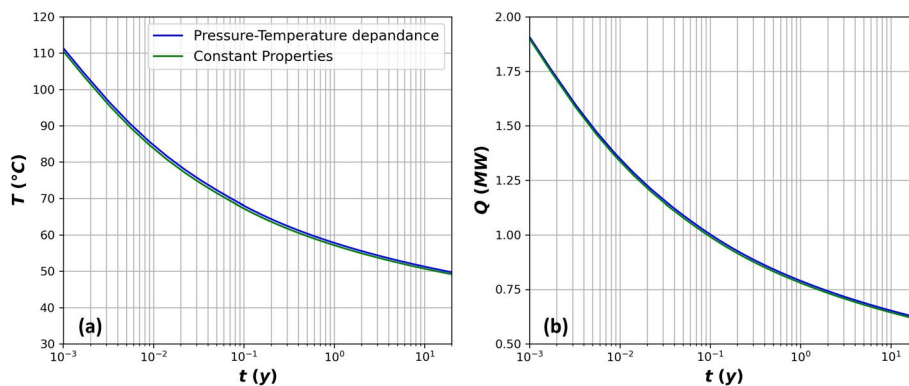
Fig. 19 Impact of water properties calculations on the a outlet temperature and b gross thermal power production ( m = 5 kg/s, T_{inj} = 20 °C)
