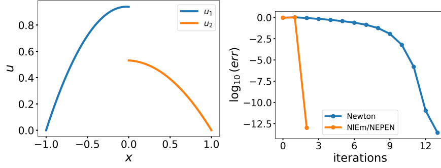
Fig. 2: Approximate solution of (20) (left) and convergence history for plane and preconditioned Newton's methods (right).
