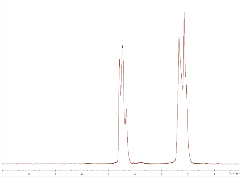
Figure S3: Pure resin by NMR-PFG diffusion 1H
